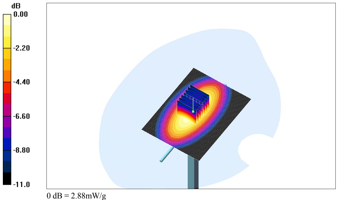
Fig. 9: 900 MHz validation result
