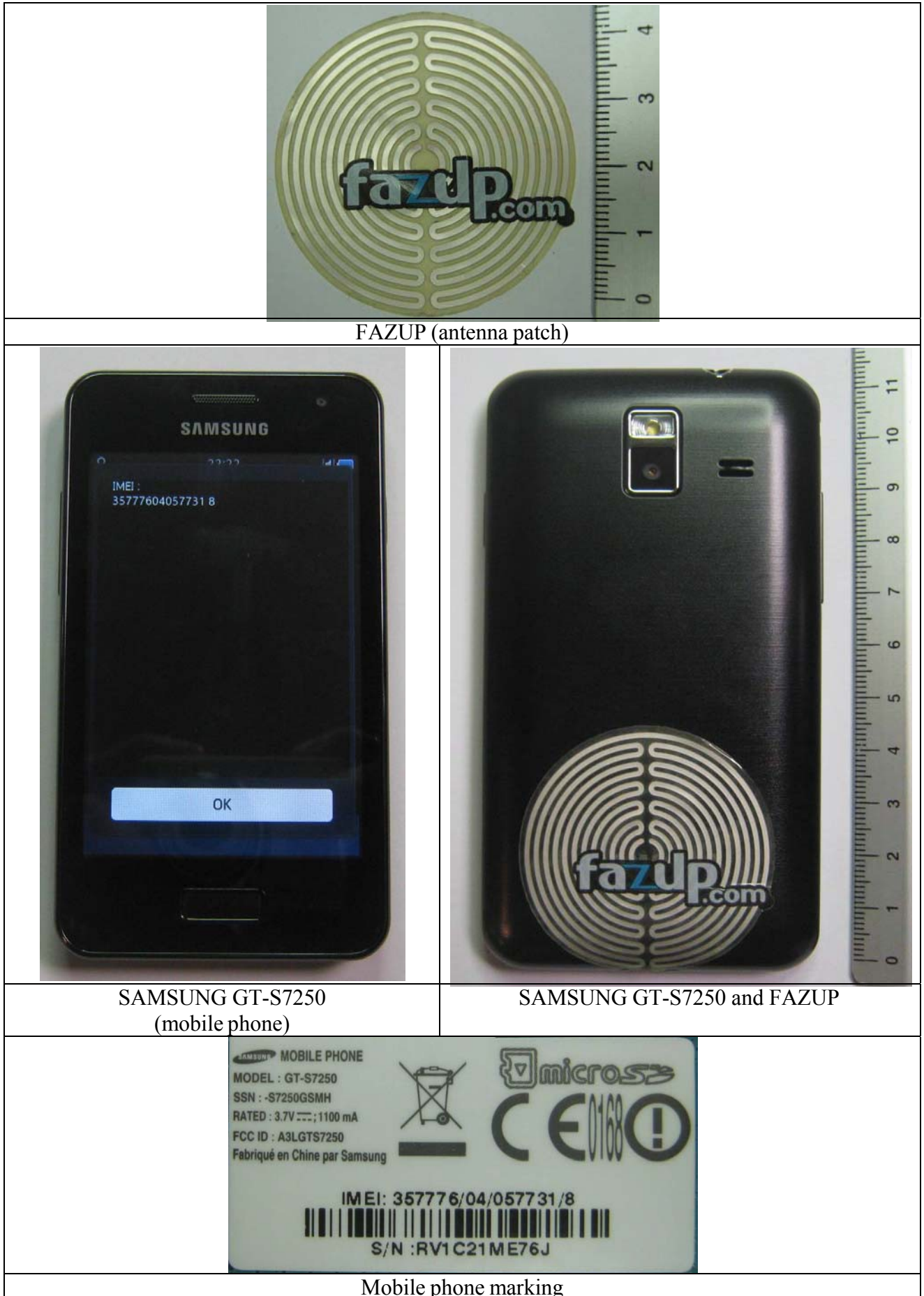
Fig. 1: Photographs of equipment under test
